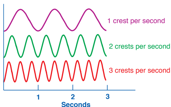
Frequency. These waves have different frequencies.
