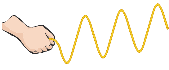
Transverse wave
