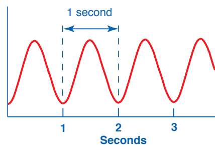
Period. This wave has a period of one second.
